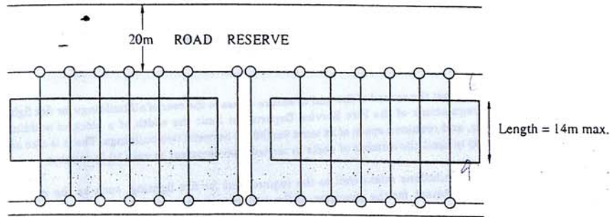
Fig. 11.1.A Permitted length of intermediate terraced residential building
