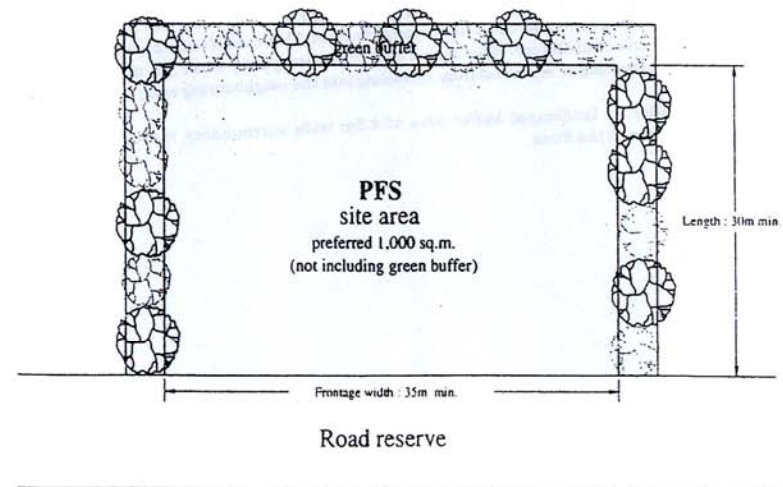
FIG. 16.3 PREFERRED PLOT SIZE OF PETROL FILLING STATION
