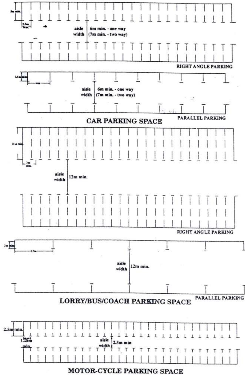
FIG. 7.2 MINIMUM DIMENSIONS OF PARKING SPACES
