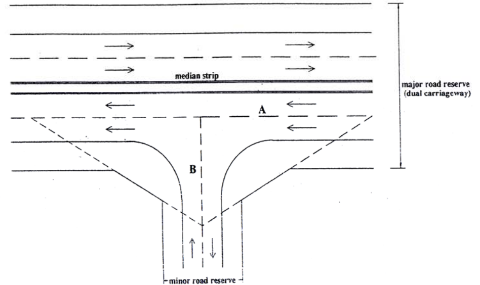
FIG. 4.1(a) TYPICAL TRUNCATION AT T-JUNCTION (DUAL CARRIAGEWAY)
