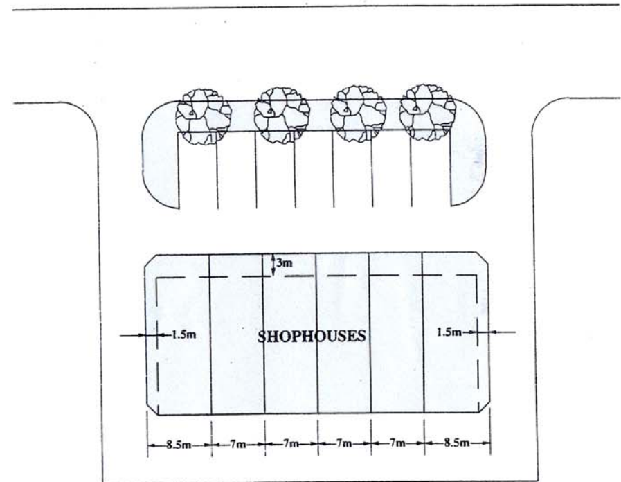
FIG. 6.2 WIDTH OF "KAKI-LIMA"
