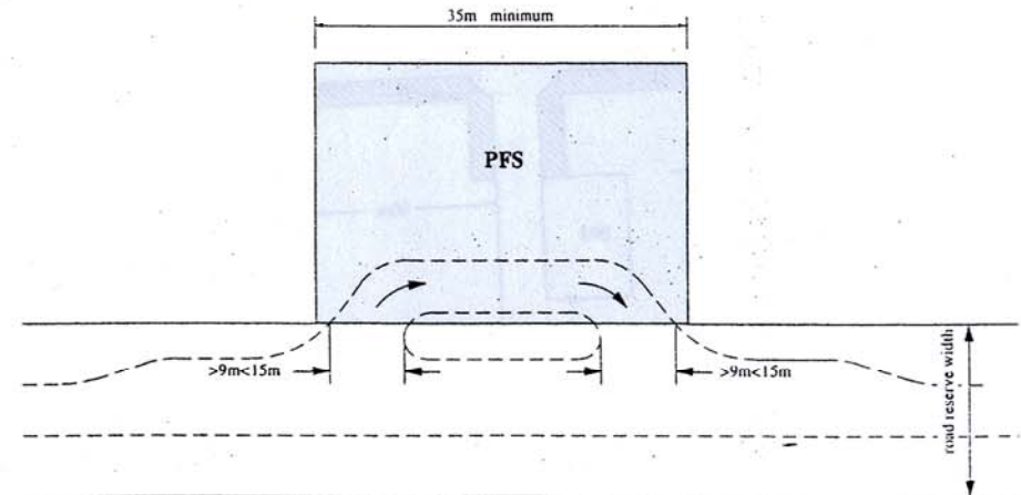
FIG. 16.5 WIDTH OF DRIVEWAY
