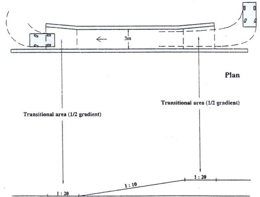
FIG. 7.3 AN EXAMPLE OF STRAIGHT RAMP (WITH 'FLAT SECTION')
