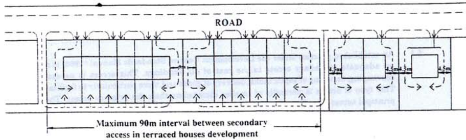
(a) Secondary access for residential
