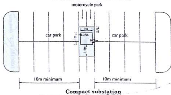
FIG. 17.1 SITING OF ELECTRICAL SUBSTATION
