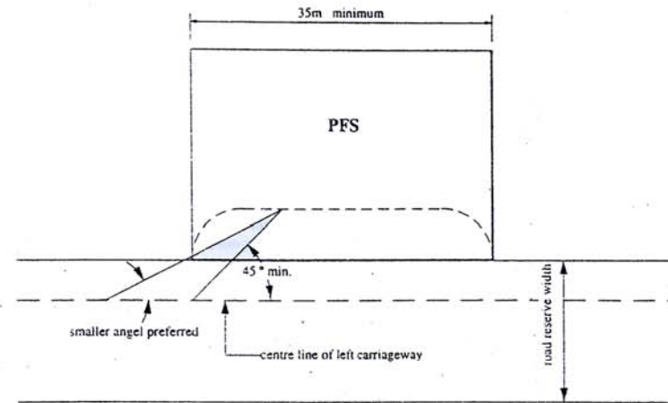
FIG. 16.4 ANGLE OF DRIVEWAY
