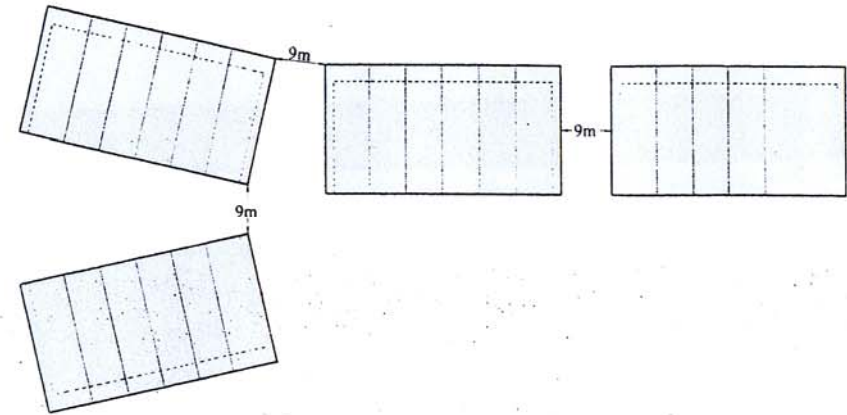
Example 1 : firebreak between shophouses
