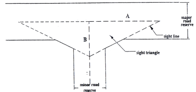
FIG. 4.1(b) TYPICAL TRUNCATION AT T-JUNCTION
