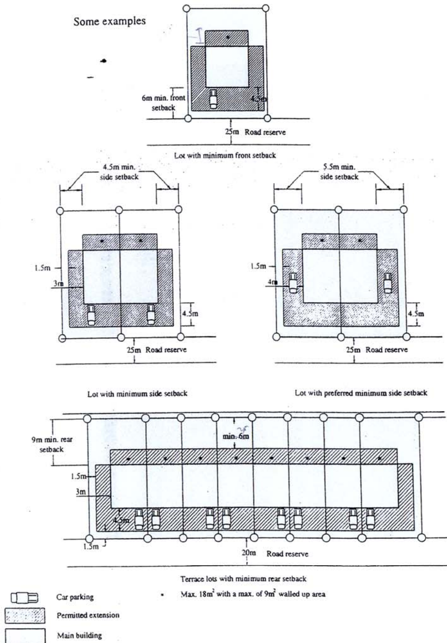
FIG. 9.1 PERMITTED EXTENSIONS IN RESIDENTIAL LOTS
