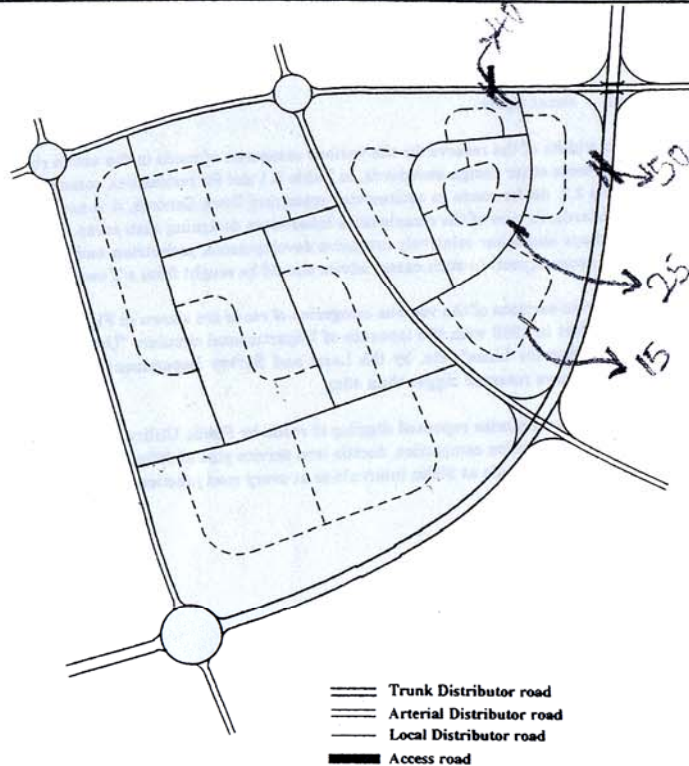
FIG. 2.1 FUNCTIONAL HIERARCHY OF URBAN ROADS
