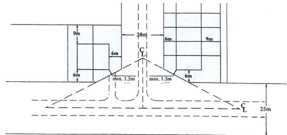
FIG. 8.1 EXAMPLE OF SETBACK FROM TRUNCATED ROAD JUNCTION
