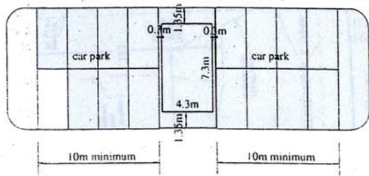
Conventional substation
