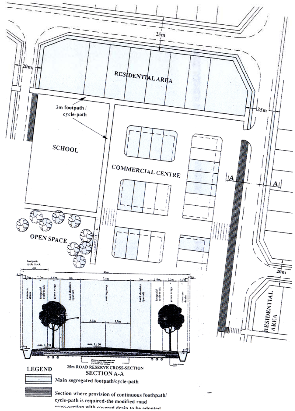
FIG. 6.1 MODIFIED ROAD CROSS-SECTION TO ACCOMMODATE CYCLE-PATH
