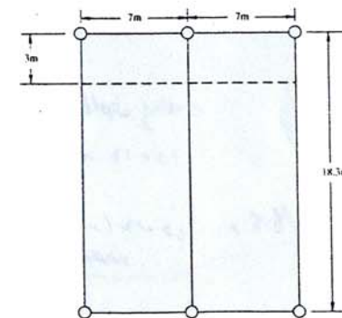
Fig.13.1.C Shophouses
