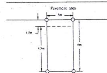
Fig.13.1.A Lock-up shop
