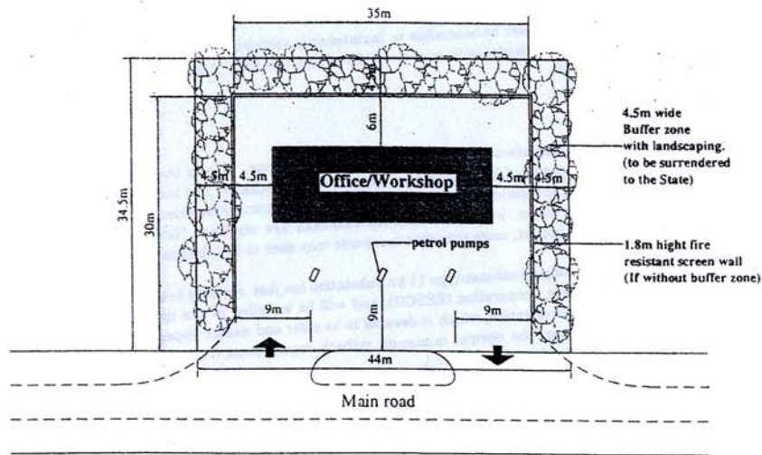
FIG. 16.6 SETBACK REQUIREMENTS OF TYPICAL PETROL FILLING STATION
